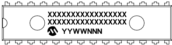
28-Lead SPDIP (.300")
