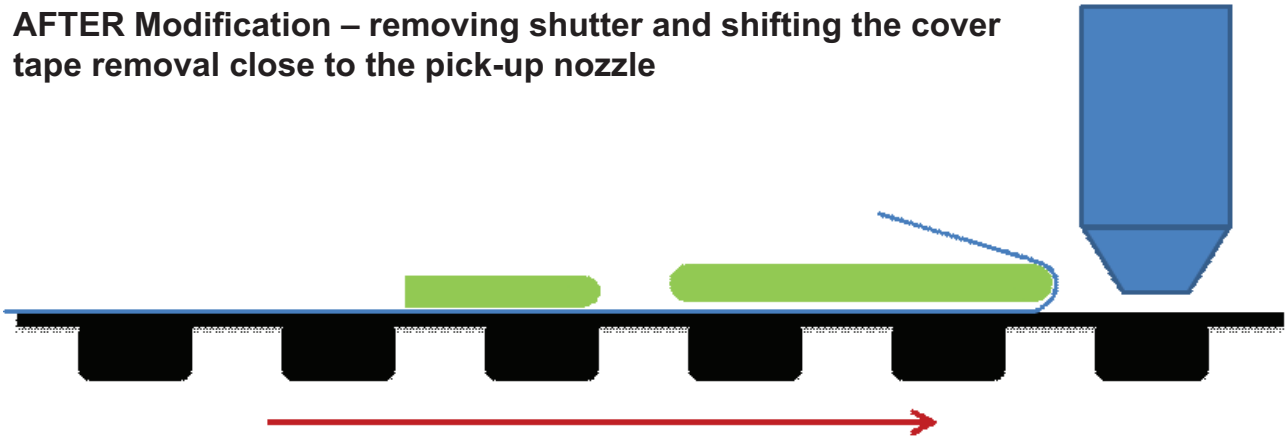
Figure 38. Minor modifications to the pick and place machine minimize the chance of damage to the dome of LUXEON Rebel.
