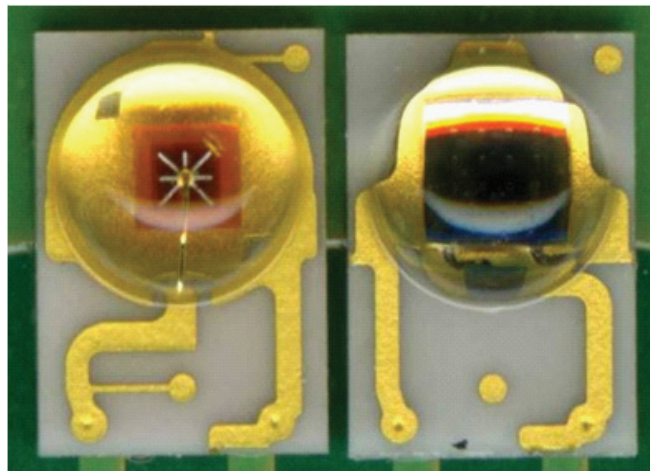
Figure 3. Picture of AlInGaP and InGaN LUXEON Rebel packages. The LUXEON Rebel AlInGaP (left) fiducials are connected to the metallization, while the LUXEON Rebel InGaN (right) has isolated fiducials.
