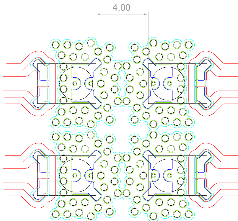
Figure 17. Illustration of edge to edge spacing. The thermal resistance will increase dramatically if the spacing is less than 4mm edge to edge.
