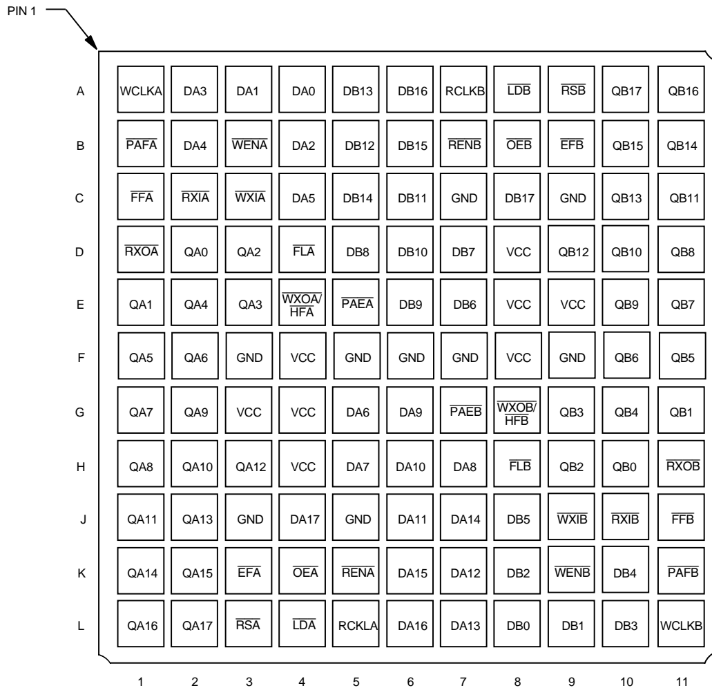
BGA (BG121-1, order code: BG) TOP VIEW
