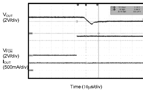
Figure 14. Mode Change Delay Time ( V_{FON} On)
