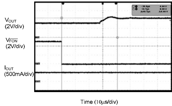
Figure 13. Mode Change Delay Time ( V_{FON} Off)
