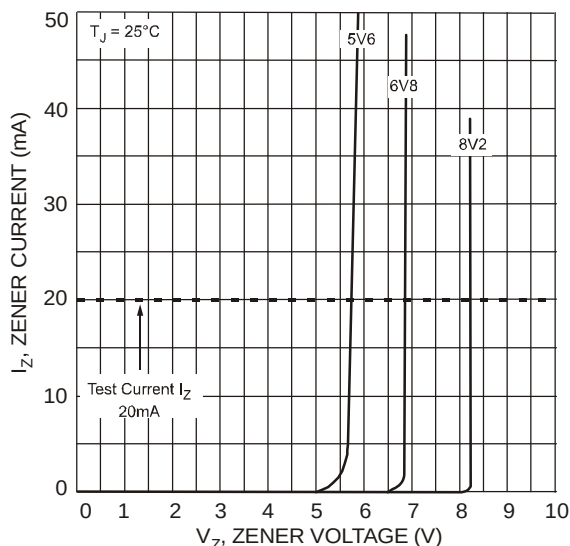
Figure 2 Typical Zener Breakdown Characteristics
