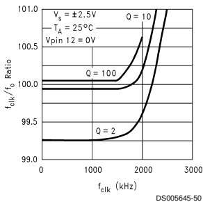
f_{\text{CLK}}/f_0 Ratio vs f_{\text{CLK}}
