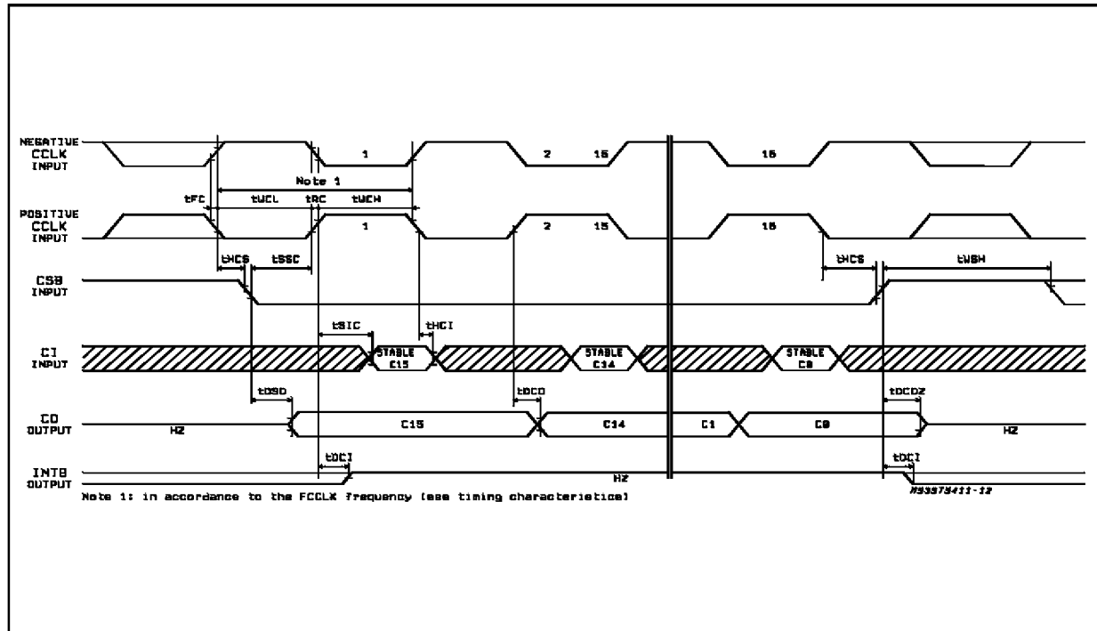
Figure 29: \mu W PORT Mode B
