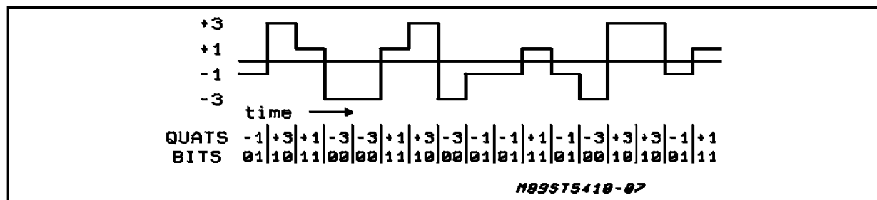
Figure 6: Example of 2B1Q Quaternary Symbols.
