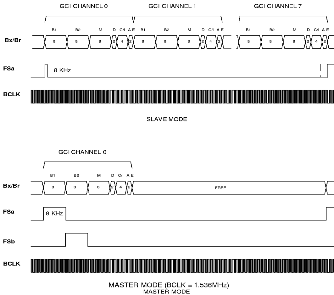
Figure 4b: GCI interface format
