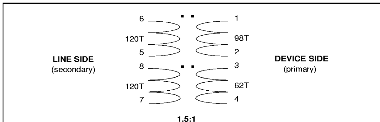
Figure 11: Transformer Design.
