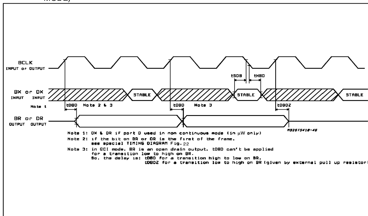
Figure 21: BX, DX, BR, DR, SLAVE & MASTER, FORMAT 4 ALWAYS NON DELAYED, ( \mu W & GCI MODE)
