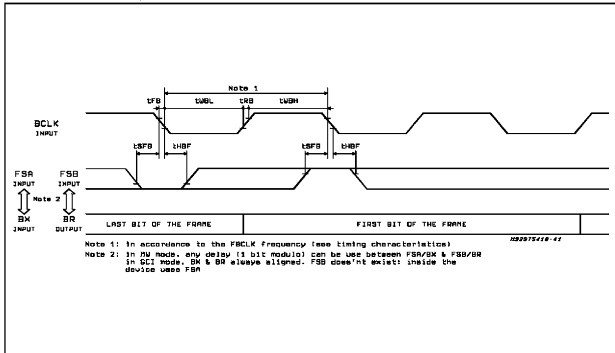
Figure 17: BCLK, FSA, FSB, MASTER MODE, DELAYED MODE, FORMATS 1 2 3 ( \mu W ONLY).
