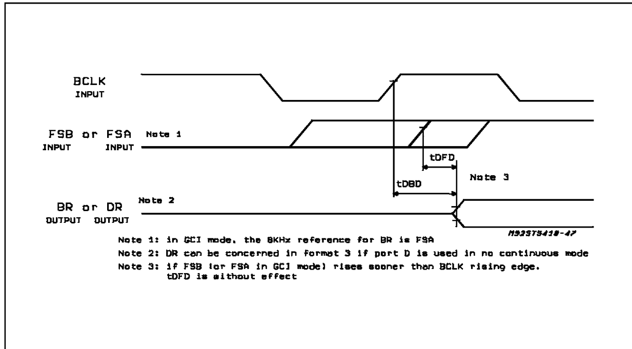
Figure 23: TSRB, SLAVE & MASTER, DELAYED & NON DELAYED, FORMATS 1 2 3 ( \mu W ONLY)
