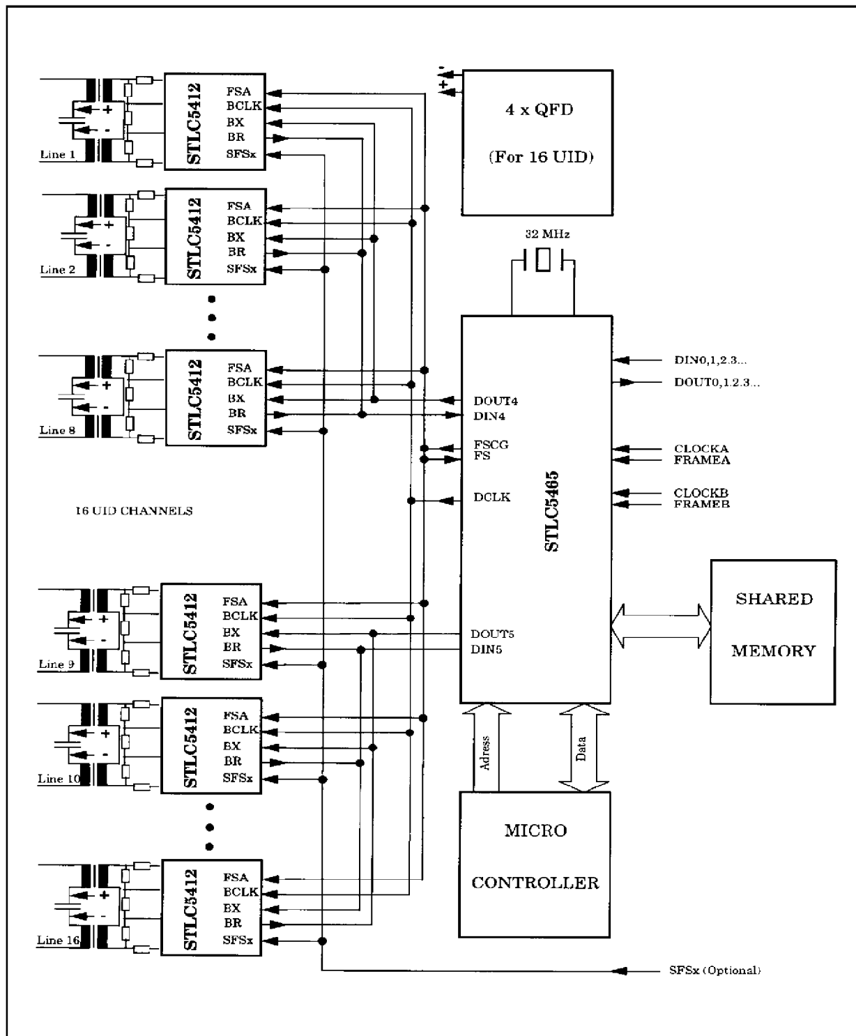
Figure 13b: LT Application.
