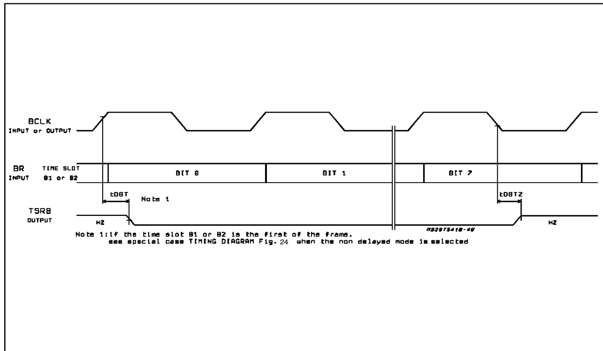
Figure 23: TSRB, SLAVE & MASTER, DELAYED & NON DELAYED, FORMATS 1 2 3 ( \mu W ONLY)
