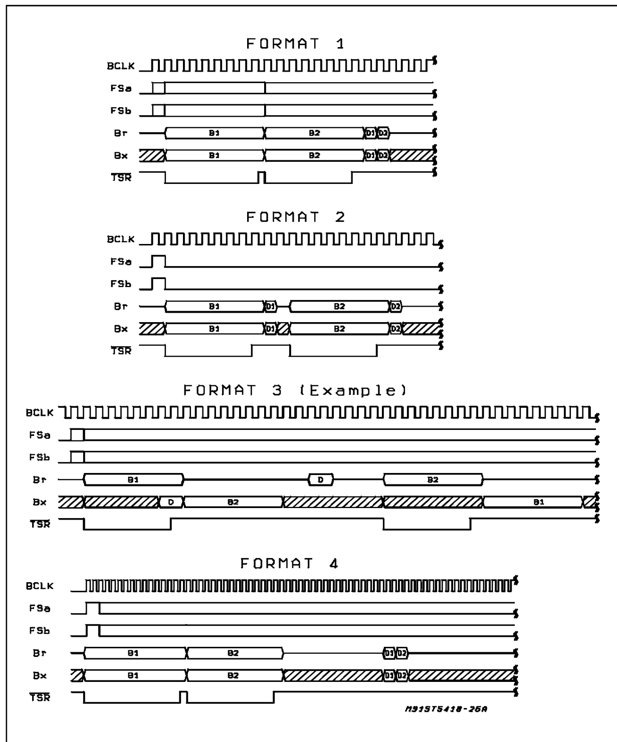
Figure 3: DSI Interface formats: SLAVE mode.
