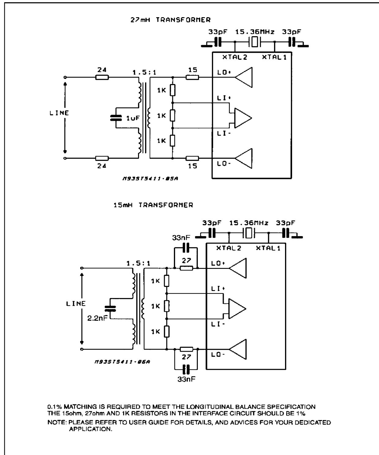
Figure 12: Recommended connections.
