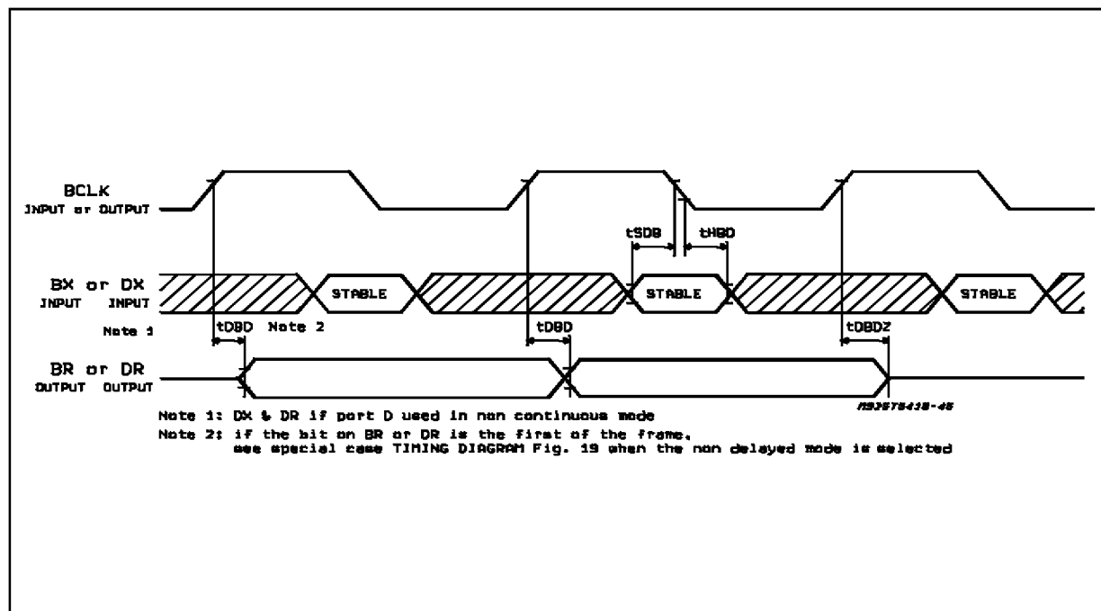
Figure 21: BX, DX, BR, DR, SLAVE & MASTER, FORMAT 4 ALWAYS NON DELAYED, ( \mu W & GCI MODE)
