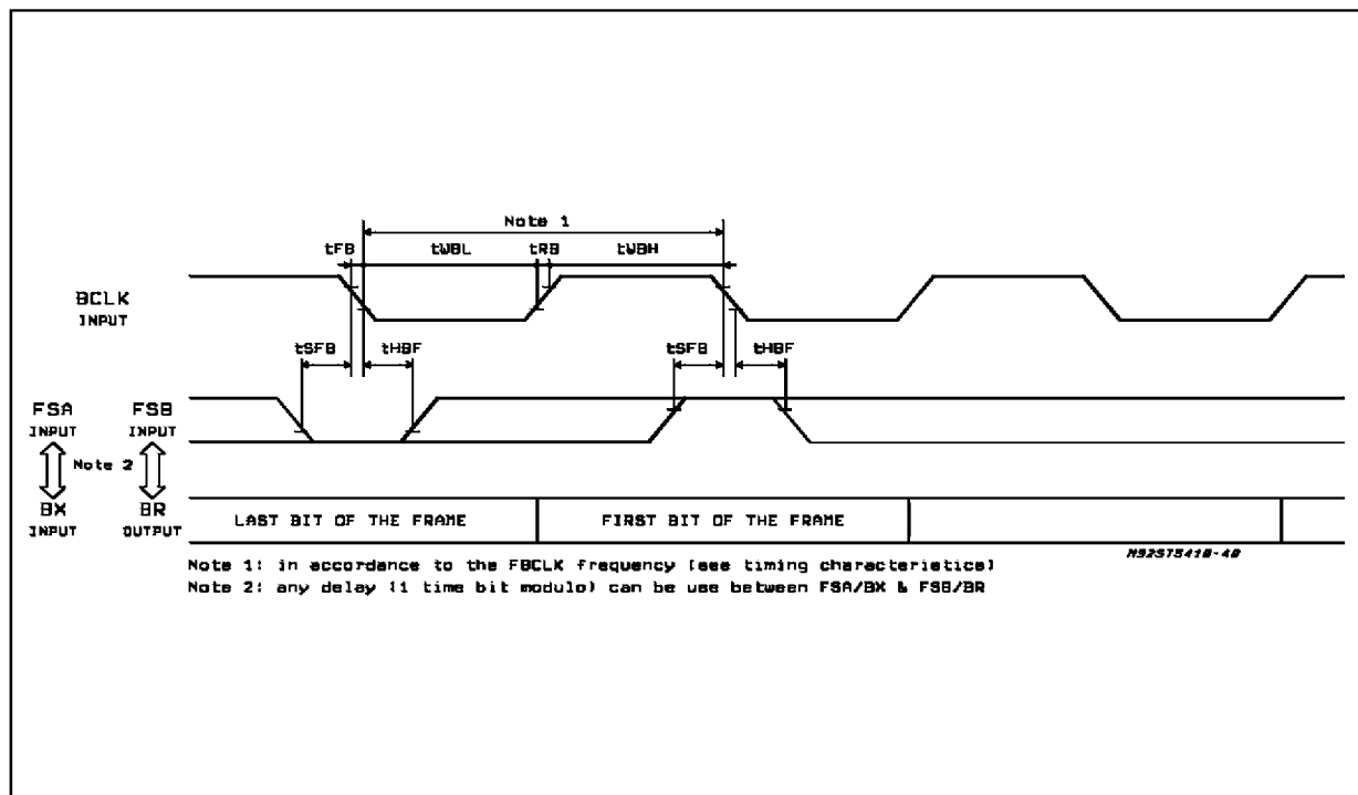
Figure 15: BCLK, FSA, FSB, SLAVE MODE, NON DELAYED MODE, FORMATS 1 2 3 ( \mu W ONLY).
