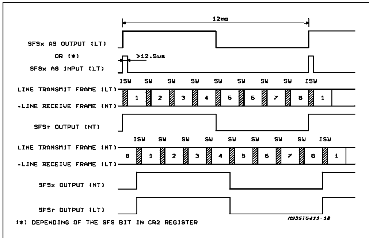
Figure 7: Superframe I/O pin SFS
