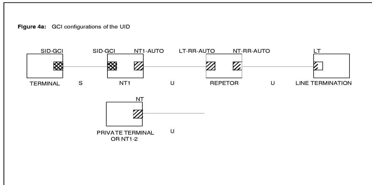
Figure 4a: GCI configurations of the UID.
