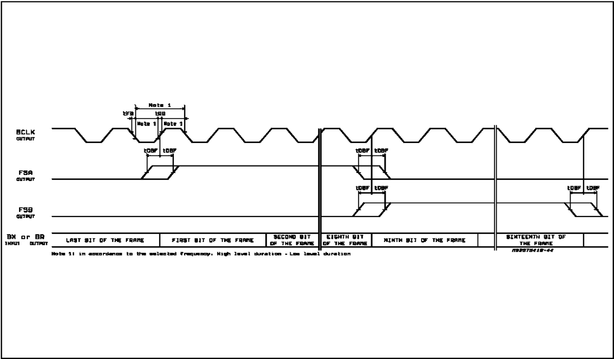
Figure 19: BCLK, FSA, FSB, MASTER MODE, FORMAT 4 ALWAYS NON DELAYED MODE, (μW AND GCI MODE).
