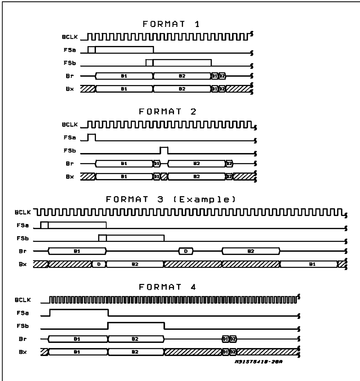
Figure 2: DSI Interface formats: MASTER mode.
