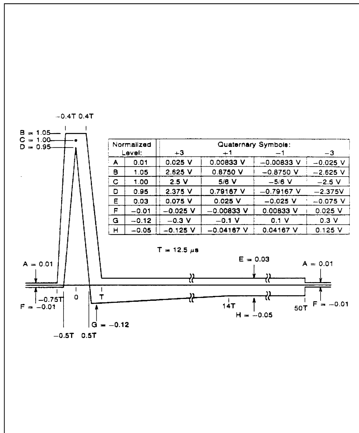
Figure 8: Normalized output pulse form
