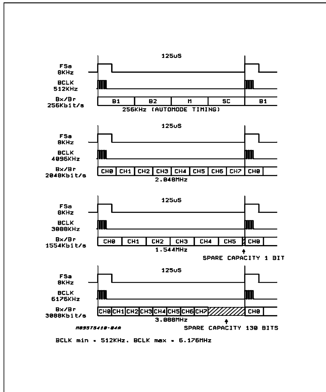
Figure 4c: GCI multiplex examples, (slave mode).
