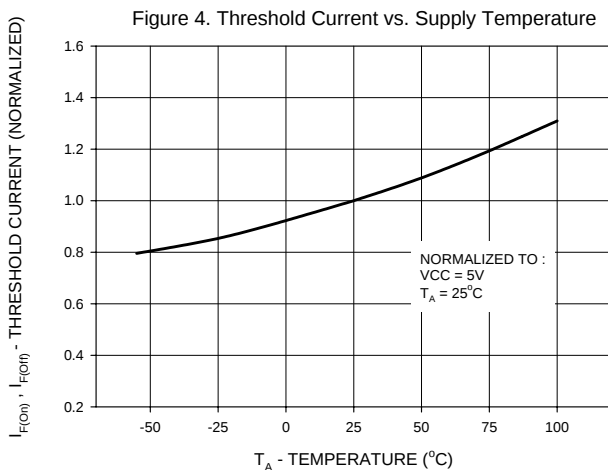
Figure 4. Threshold Current vs. Supply Temperature
