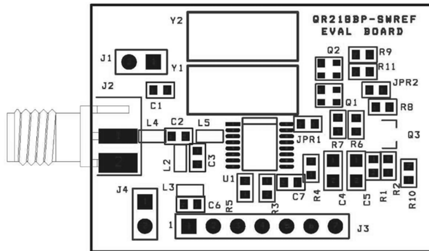
Figure 5. MICR218 Dual Frequency Evaluation Board
