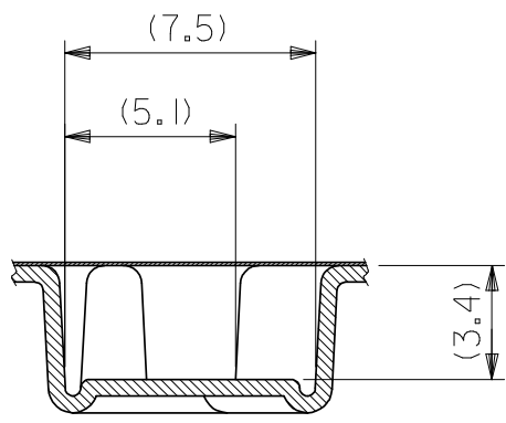
SECT:X-X (SCALE 4:1)
