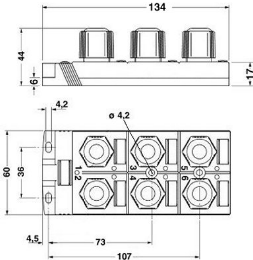
Dimensioned drawing
