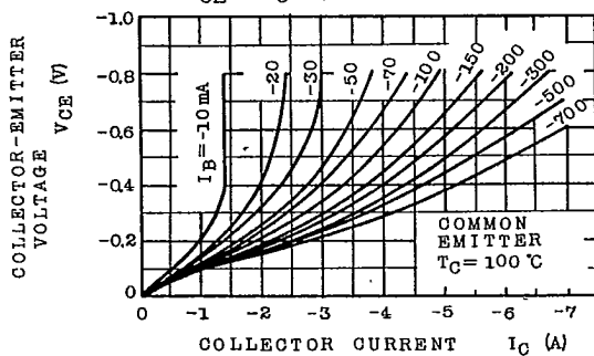
V_{CE} - I_C (LOW VOLTAGE REGION)
