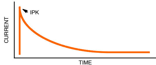
Figure 31. Input Charge Inrush Current
