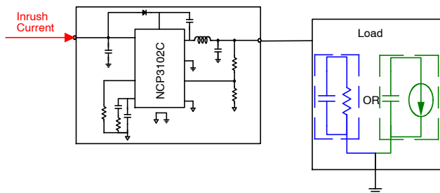
Figure 32. Load Connected to the Output Stage
