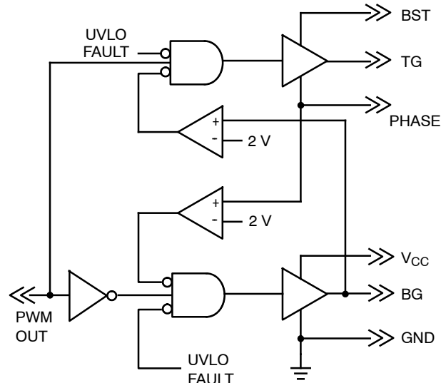
Figure 24. Block Diagram
