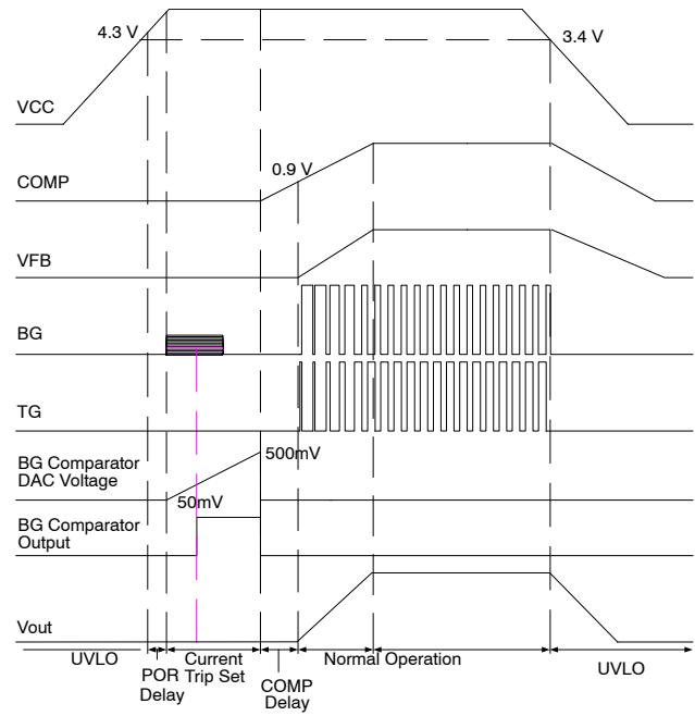
Figure 22. Soft-Start Sequence
