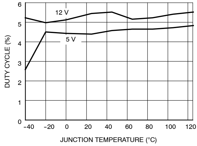
Figure 16. Minimum Duty Cycle vs. Temperature
