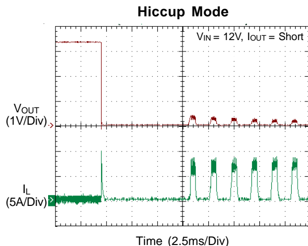
Figure 7. Hiccup Mode Under Voltage Protection
