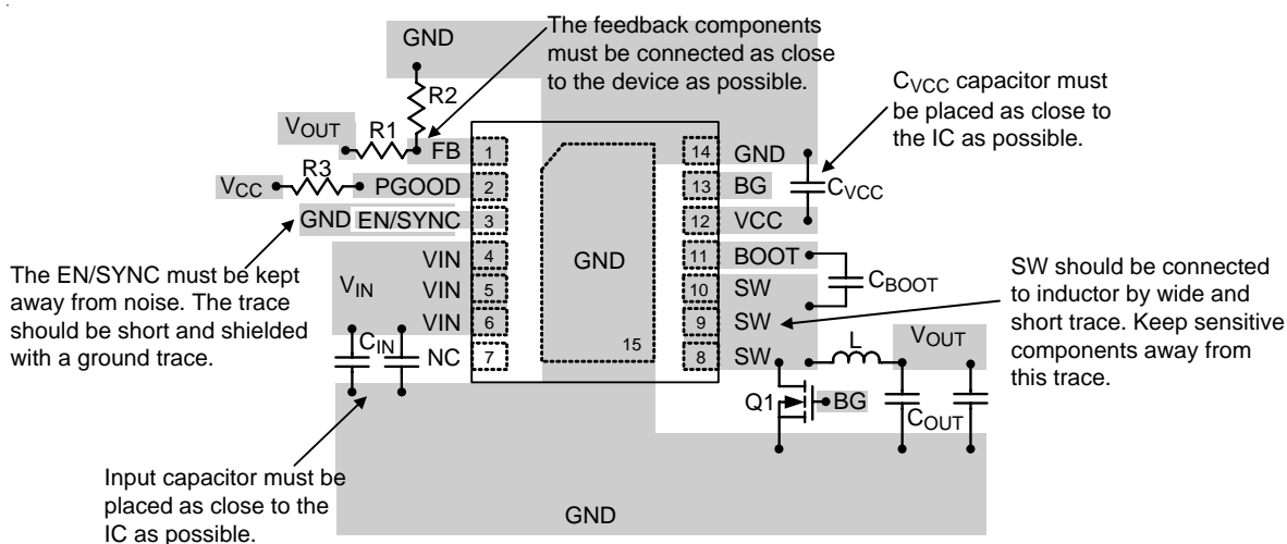
Figure 10. PCB Layout Guide for WDFN-14L 4x3
