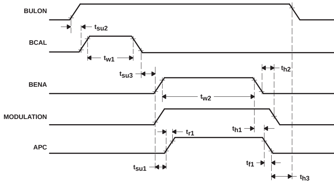
Figure 3–1. Uplink Timing Diagram
