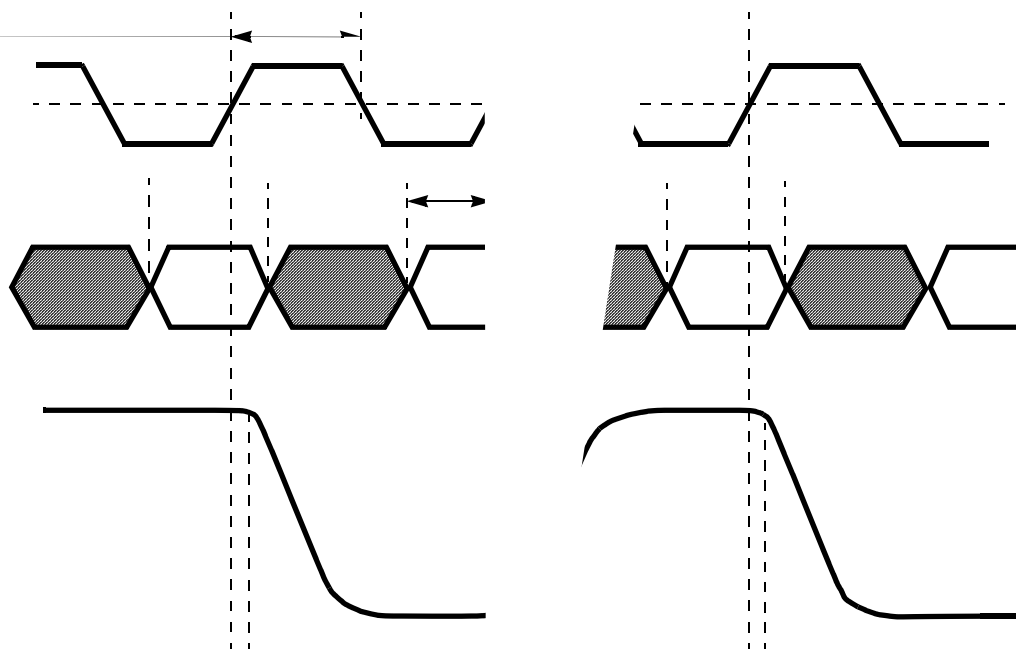
FIGURE 3. PROPAGATION DELAY, SETUP TIME, HOLD TIME AND MINIMUM PULSE WIDTH DIAGRAM
