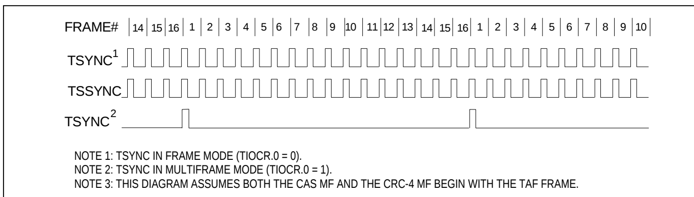
Figure 10-19. E1 Transmit-Side Timing
