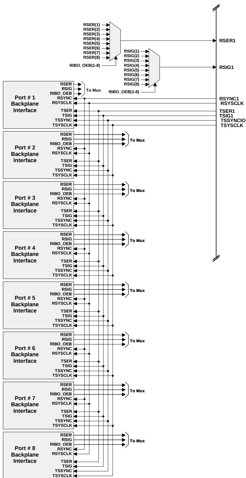
Figure 8-5. IBO Multiplexer Equivalent Circuit—16.384MHz
