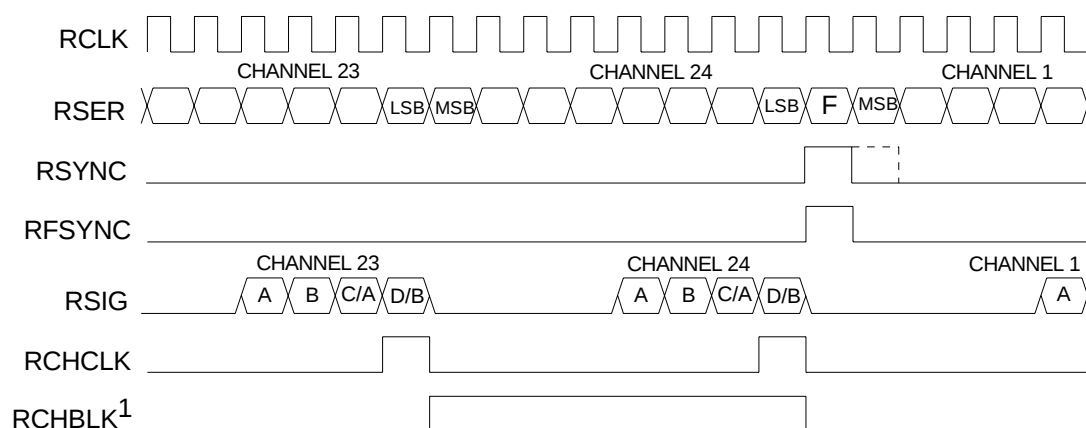
Figure 10-3. T1 Receive-Side Boundary Timing (Elastic Store Disabled)
