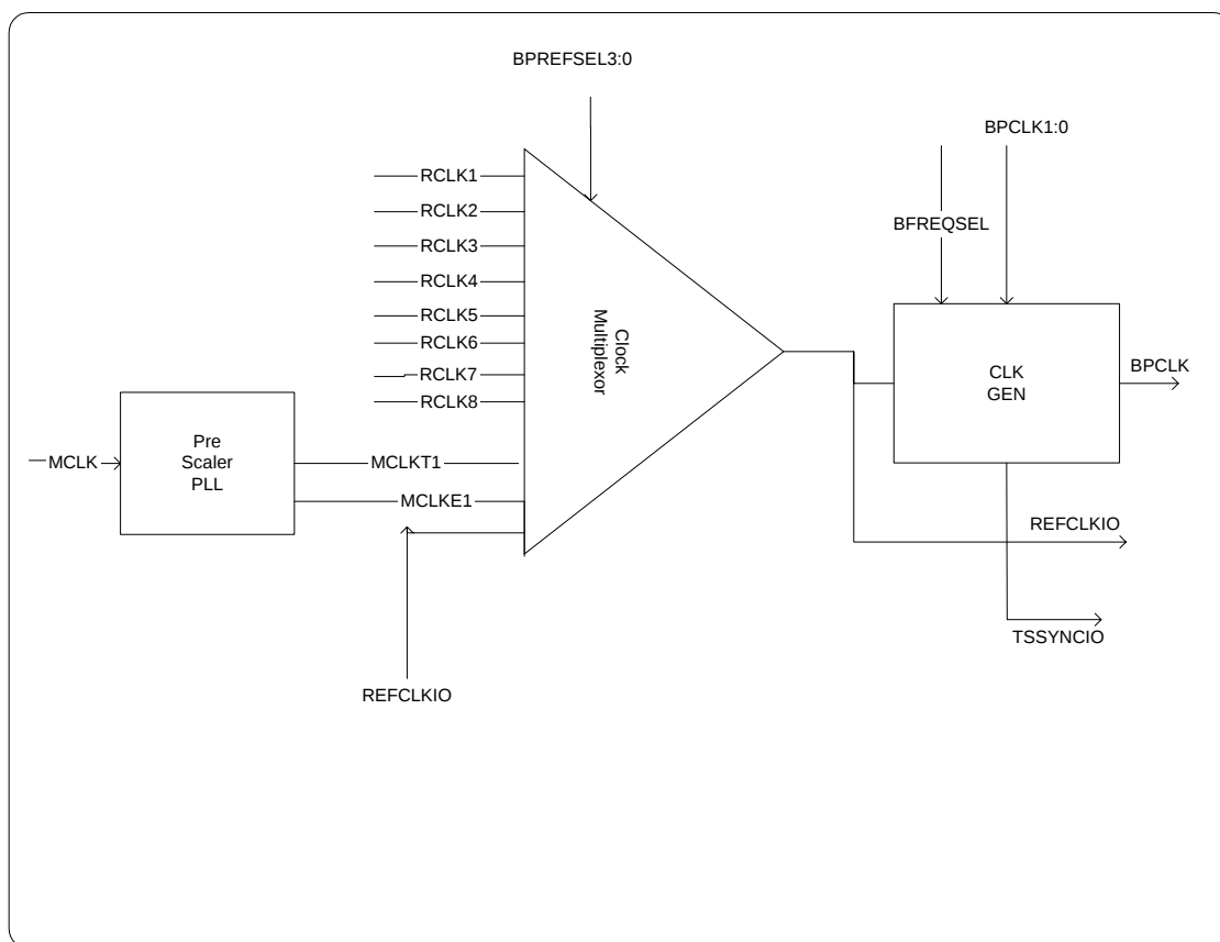
Figure 8-1. Backplane Clock Generation
