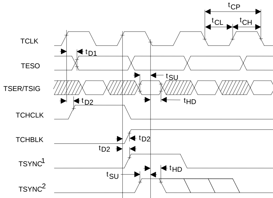
Figure 12-8. Transmit Formatter Timing—Backplane
