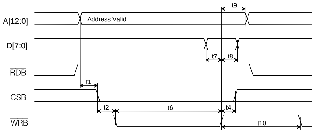
Figure 12-2. Intel Bus Write Timing (BTS = 0)
