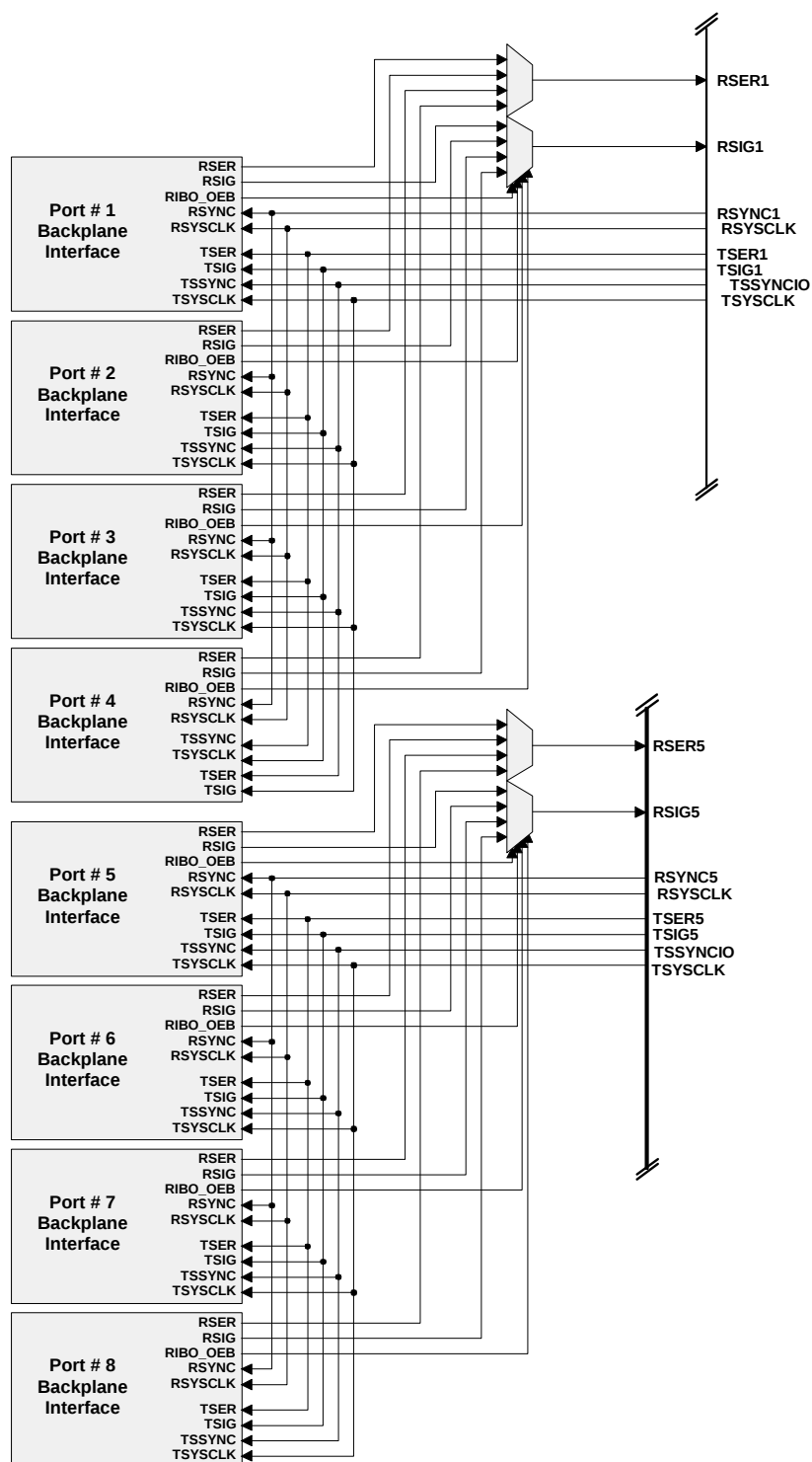
Figure 8-4. IBO Multiplexer Equivalent Circuit—8.192MHz
