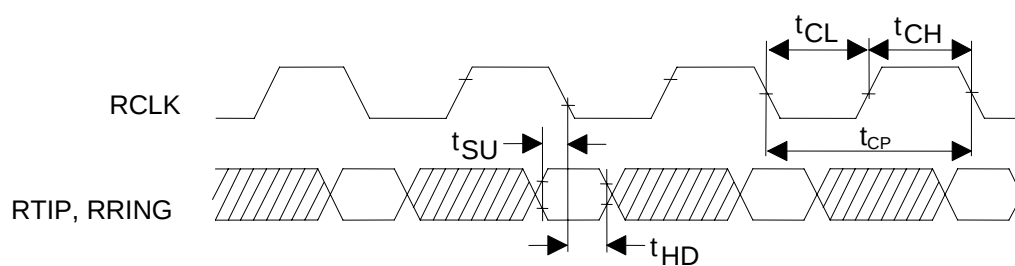
Figure 12-7. Receive Framer Timing—Line Side
