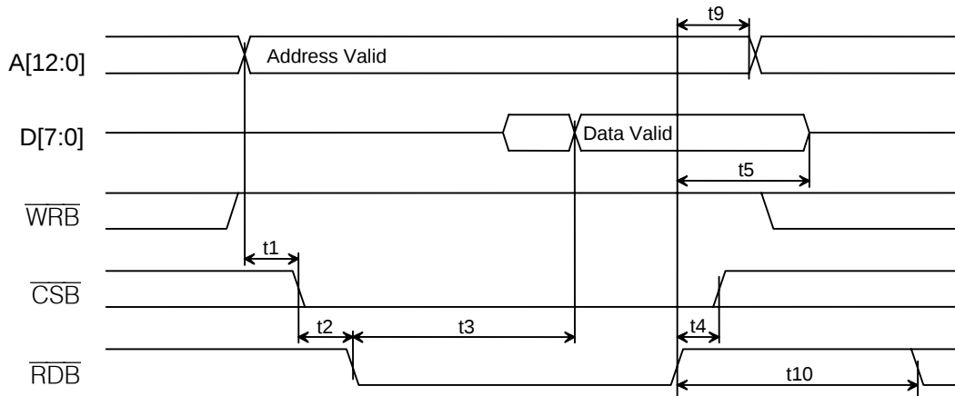
Figure 12-1. Intel Bus Read Timing (BTS = 0)
