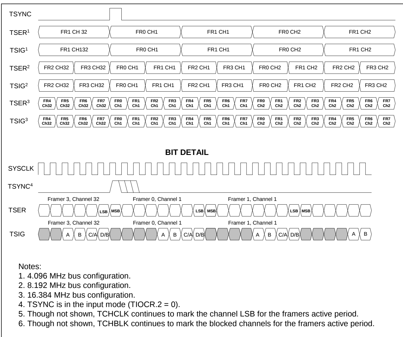
Figure 10-13. T1 Transmit-Side Interleave Bus Operation—BYTE Mode
