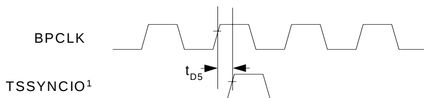
Figure 12-10. BPCLK Timing
