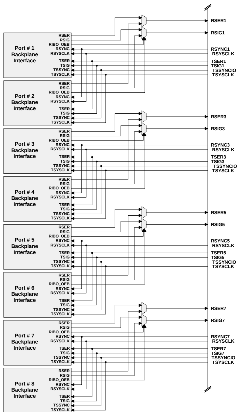
Figure 8-3. IBO Multiplexer Equivalent Circuit—4.096MHz
