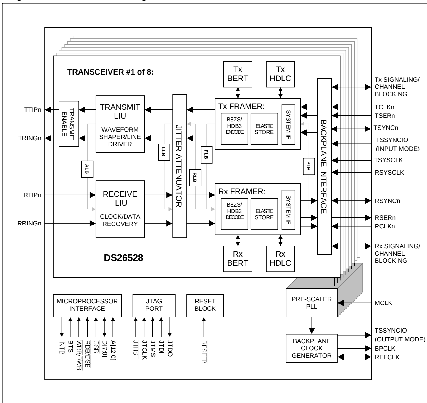
Figure 6-2. Detailed Block Diagram
