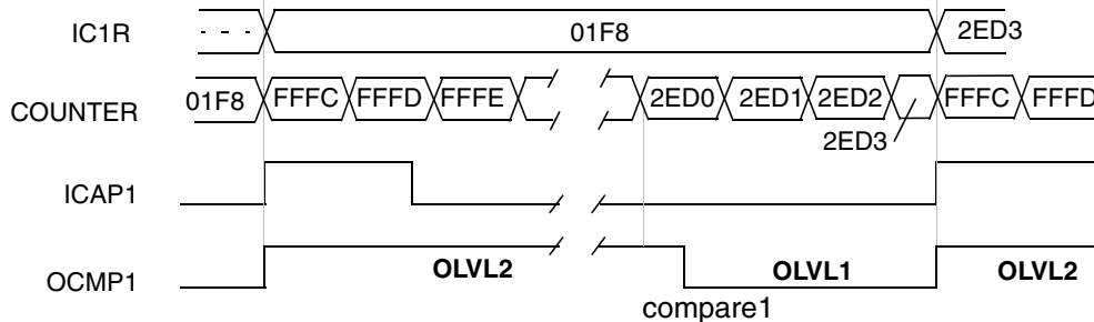
Figure 44. One Pulse Mode Timing Example
