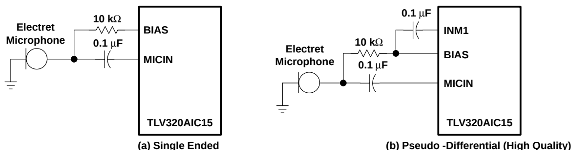
Figure 3–1. Microphone Interface
