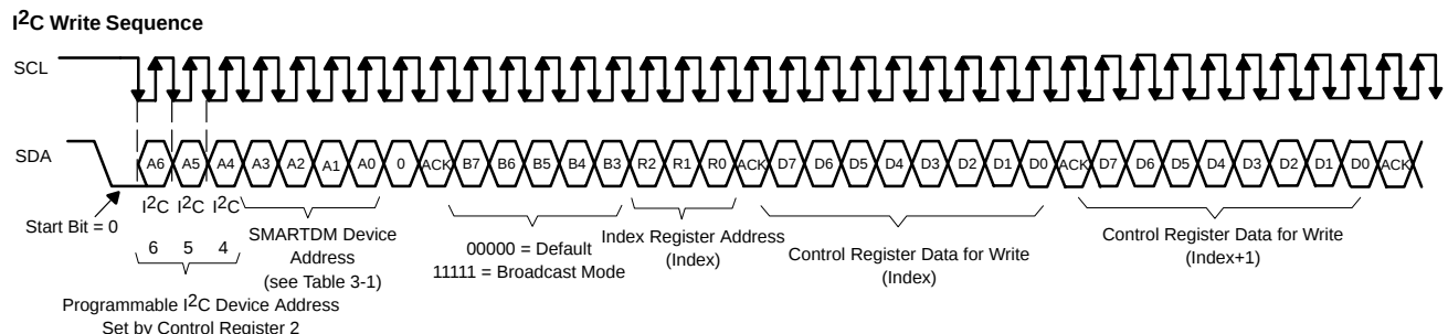
Figure 3–10. I 2 C Write Sequence
