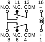
Tolerance: ±0.1 ± .004 Schematic (Bottom view)
