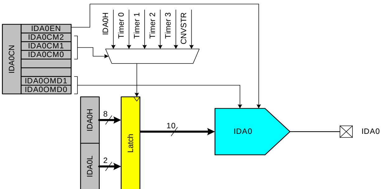
Figure 1.10. IDA0 Functional Block Diagram
