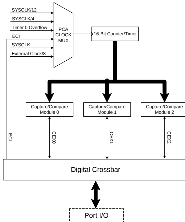
Figure 1.7. PCA Block Diagram
