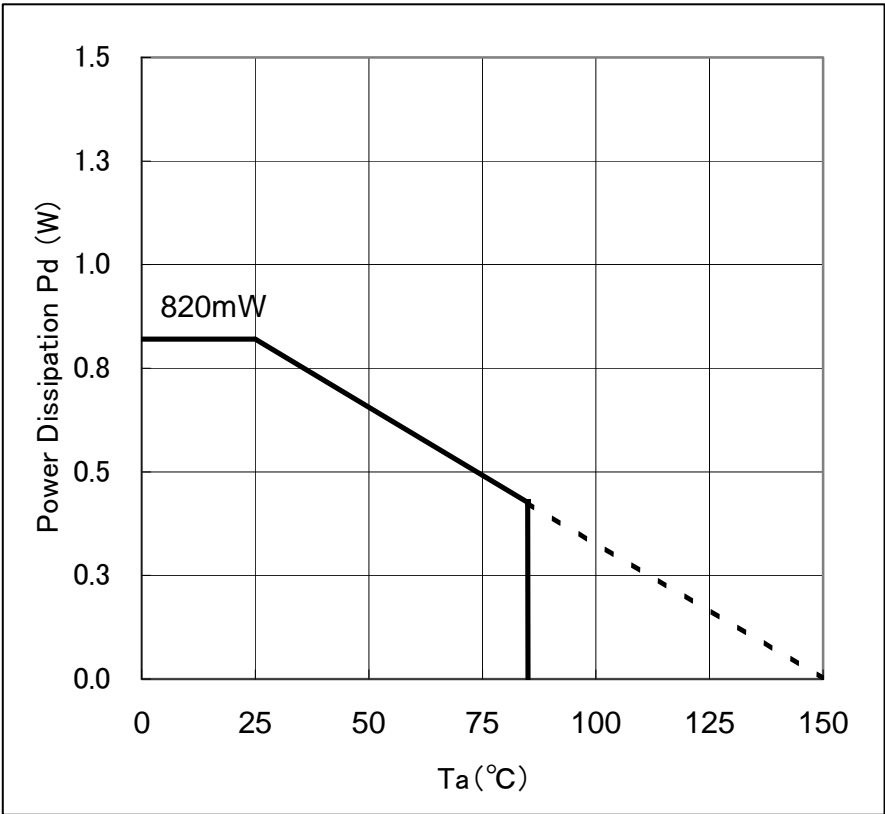
Figure 33. Power dissipation
