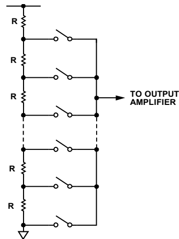
Figure 58. Resistor String
