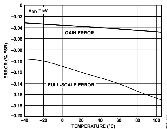
Figure 30. Gain Error and Full-Scale Error vs. Temperature
