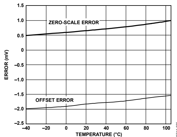
Figure 31. Zero-Scale Error and Offset Error vs. Temperature
