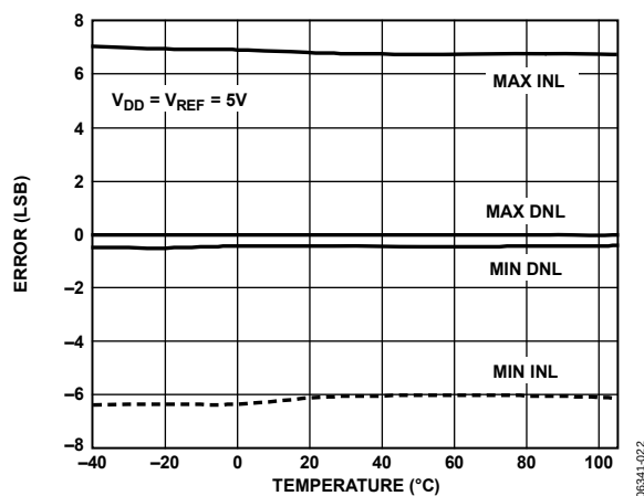
Figure 27. INL Error and DNL Error vs. Temperature
