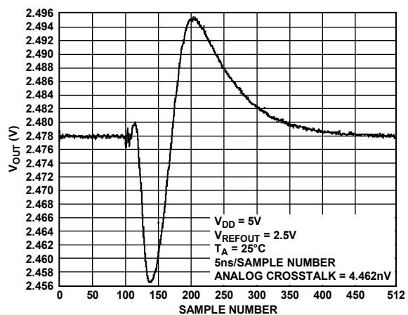
Figure 47. Analog Crosstalk, Internal Reference
