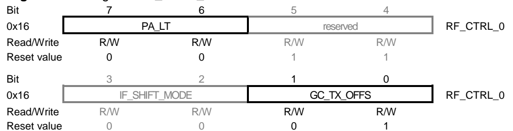
Figure 9-15. Register RF_CTRL_0.
