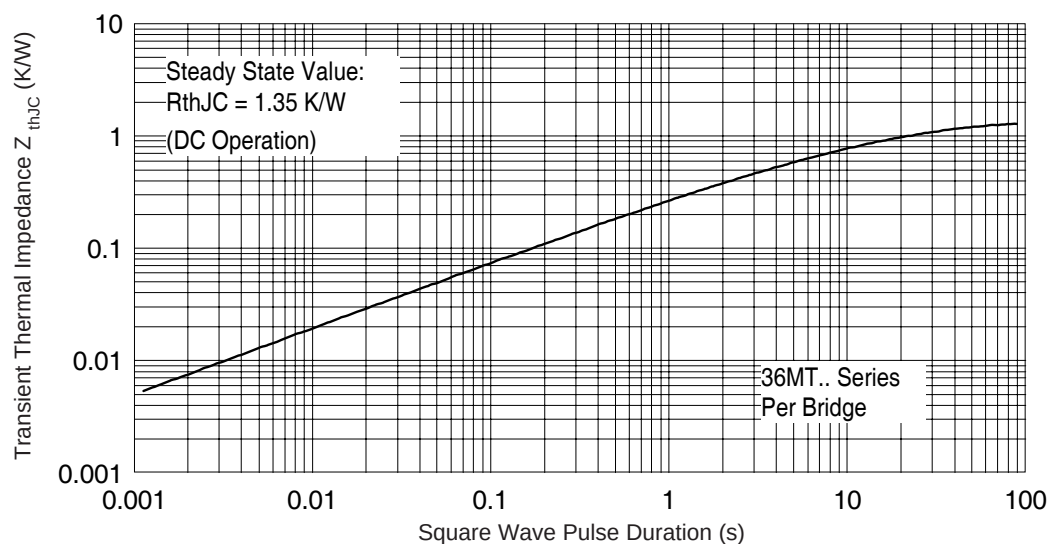
Fig. 12 - Thermal Impedance Z_{thJC} Characteristics
