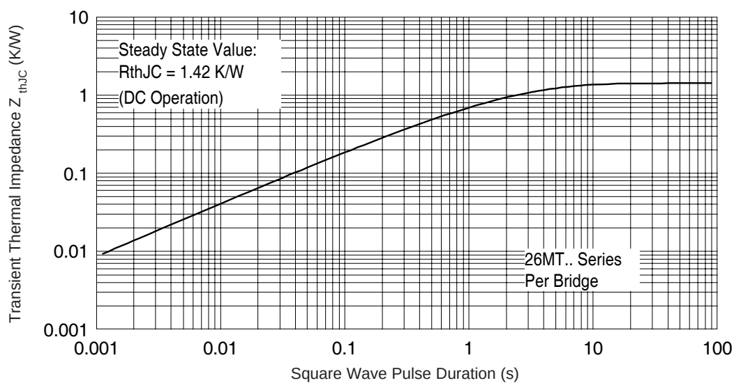
Fig. 11 - Thermal Impedance Z_{thJC} Characteristics
