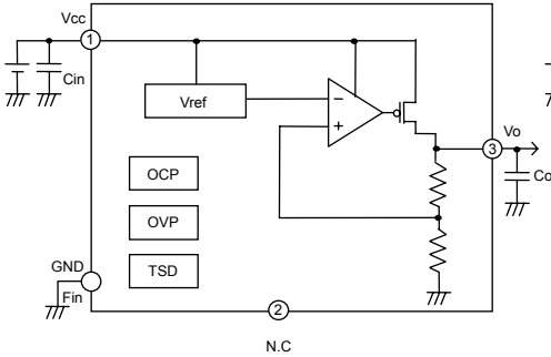
Fig.13 TO252-3
