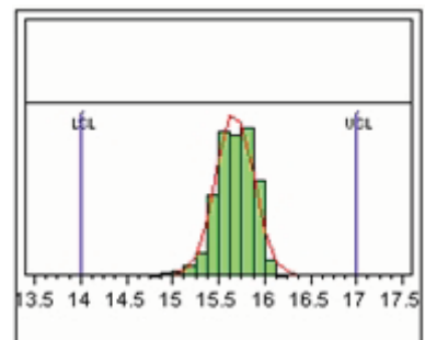
Figure 4. Gain @ 0.6GHz 3V 10mA, LSL=14.25, Nominal=15.70, USL=17.25
