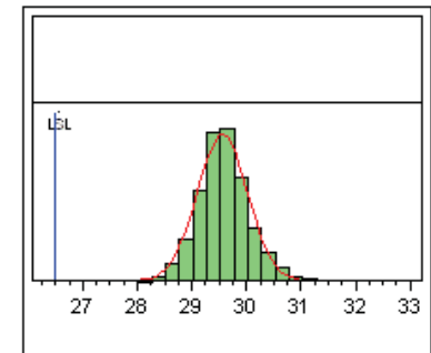
Figure 7. IIP3_bypass @ 0.6GHz 3V 0mA, LSL=26.5, Nominal=29.5
