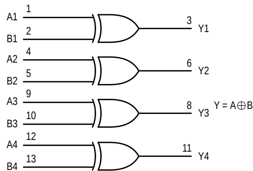
LOGIC DIAGRAM
