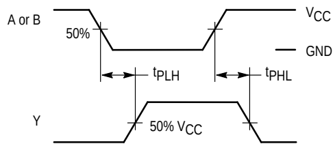
Figure 1. Switching Waveforms
