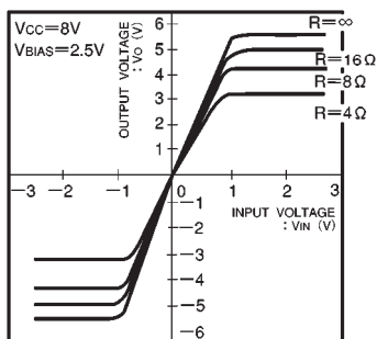
Fig.8 Driver (channel 3) I/O characteristics (variable load)
