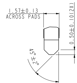
DETAIL A SCALE 5:1
