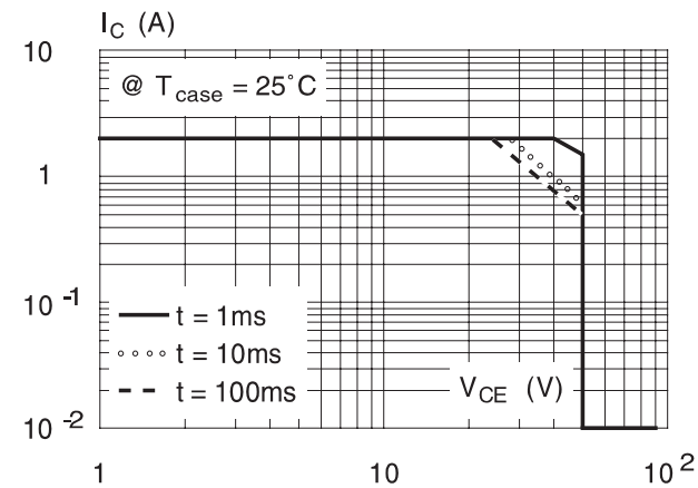
Figure 2. Output transistors SOA (for secondary breakdown)
