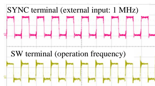
Fig.24 External synchronization operation
