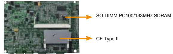
Solder Side
