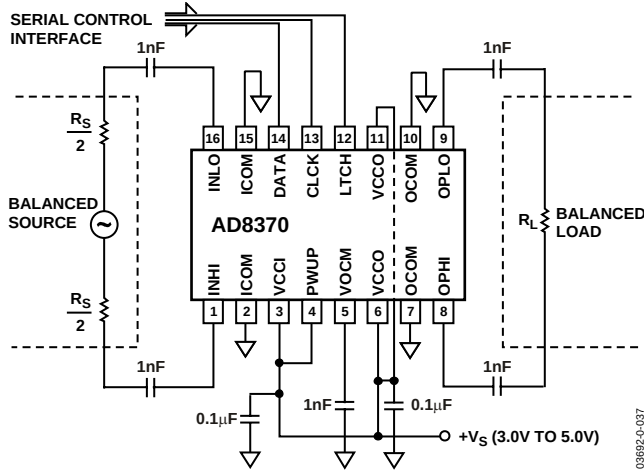
Figure 42. Basic Connections
