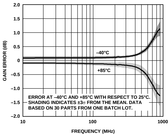
Figure 12. Gain Error over Temperature vs. Frequency, R_L = 100\text{ }\Omega
