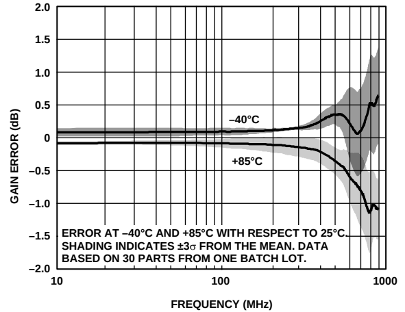
Figure 15. Gain Error over Temperature vs. Frequency, R_L = 1\text{ k}\Omega
