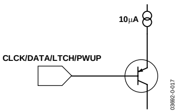
Figure 40. Simplified Circuit for Digital Inputs
