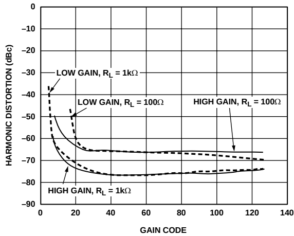
Figure 16. Second-Order Harmonic Distortion vs. Gain Code at 70 MHz, V_{OUT} = 2\text{ V p-p Differential}
