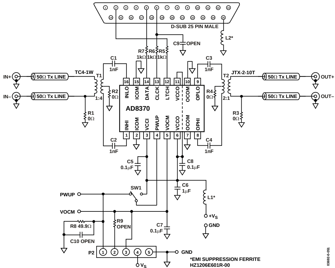
Figure 57. AD8370 Evaluation Board Schematic
