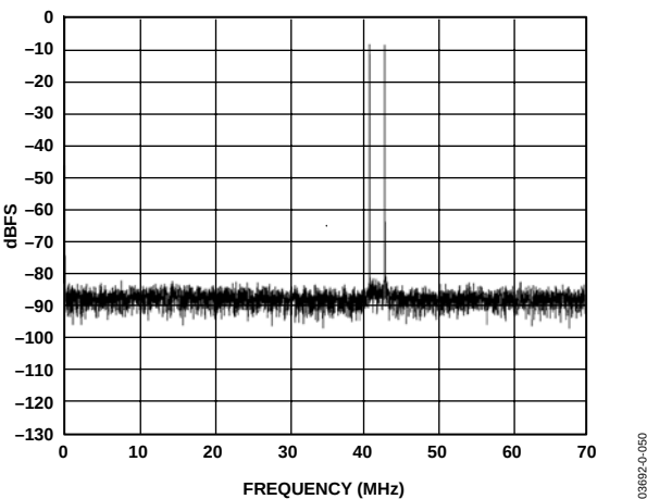
Figure 55. FFT Plot of Two-Tone Intermodulation Distortion at 42 MHz for the Circuit in Figure 56
