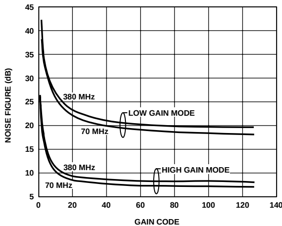
Figure 6. Noise Figure vs. Gain Code at 70 MHz
