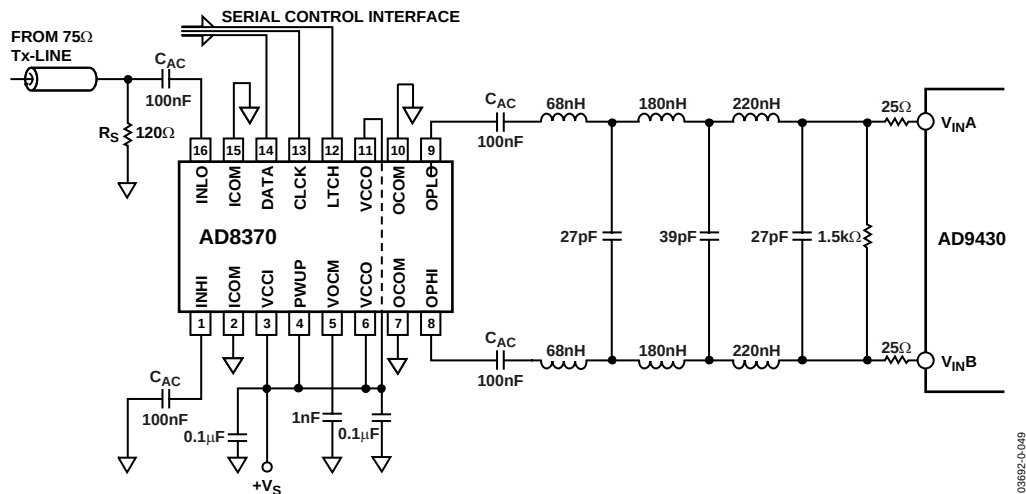
Figure 56. ADC Interface Example
