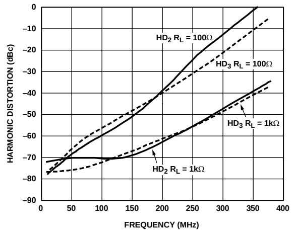
Figure 20. Harmonic Distortion vs. Frequency at Maximum Gain, V_{OUT} = 2\text{ V p-p Composite Differential}
