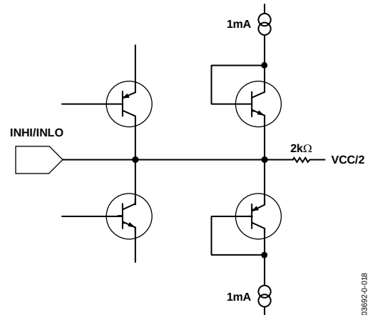
Figure 36. INHI/INLO Simplified Schematic
