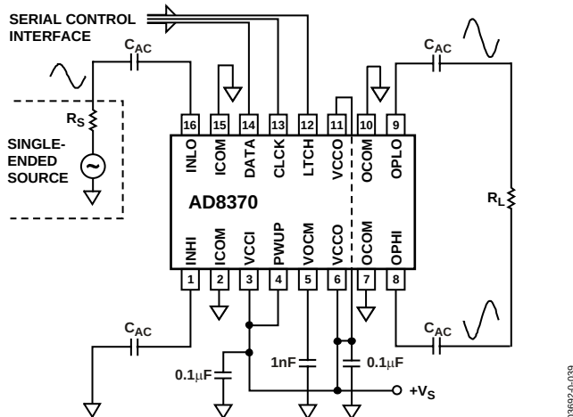
Figure 45. Single-Ended-to-Differential Conversion
