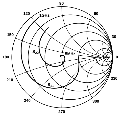
Figure 17. Input and Output Reflection Coefficients, S_{11} and S_{22} , Z_O = 100\ \Omega Differential
