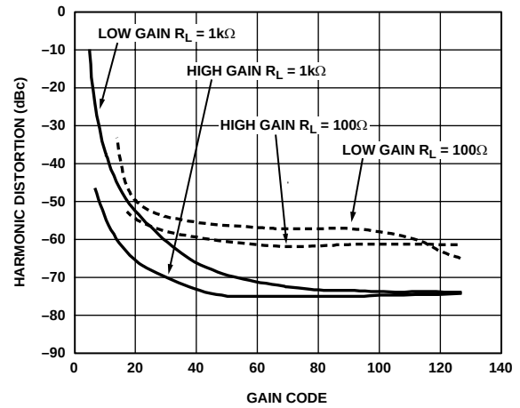
Figure 19. Third-Order Harmonic Distortion vs. Gain Code at 70 MHz, V_{OUT} = 2\text{ V p-p Differential}
