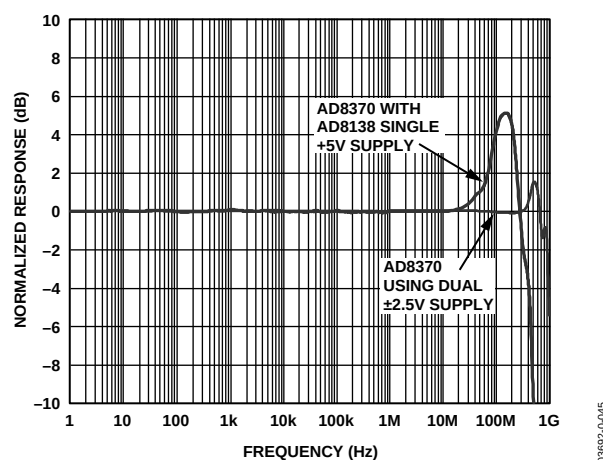
Figure 51. Normalized Frequency Response of the Two Solutions in Figure 49 and Figure 50
