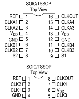
Pin Configuration
