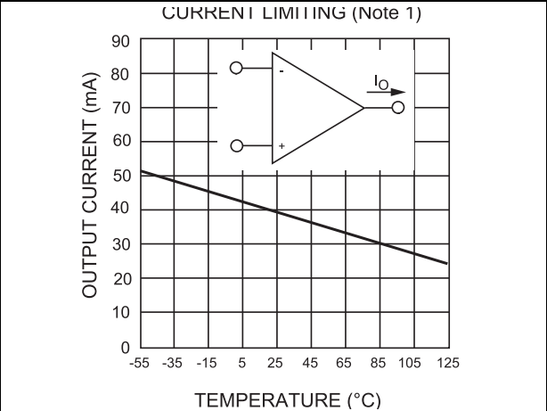
Figure 9. Current limiting
