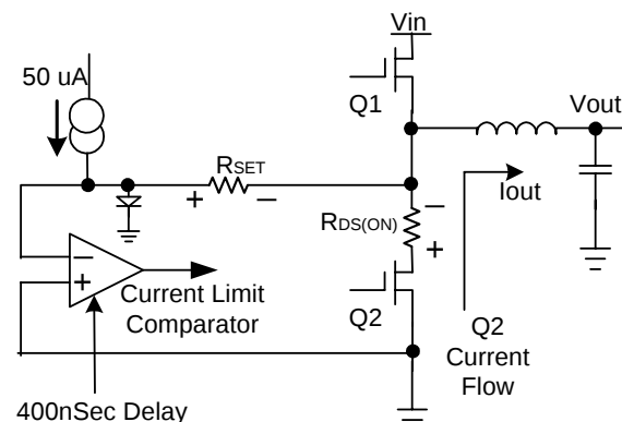
Figure 3 – Phase 1 \bar{I} Current Limit
