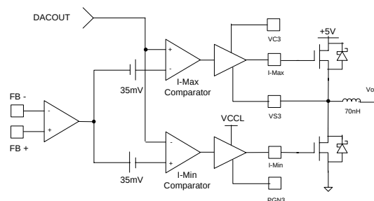
Figure 6 – Phase 3 Transient Correction Loop
