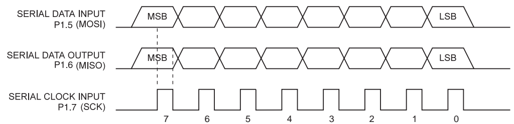
Figure 13. Serial Programming Waveforms
