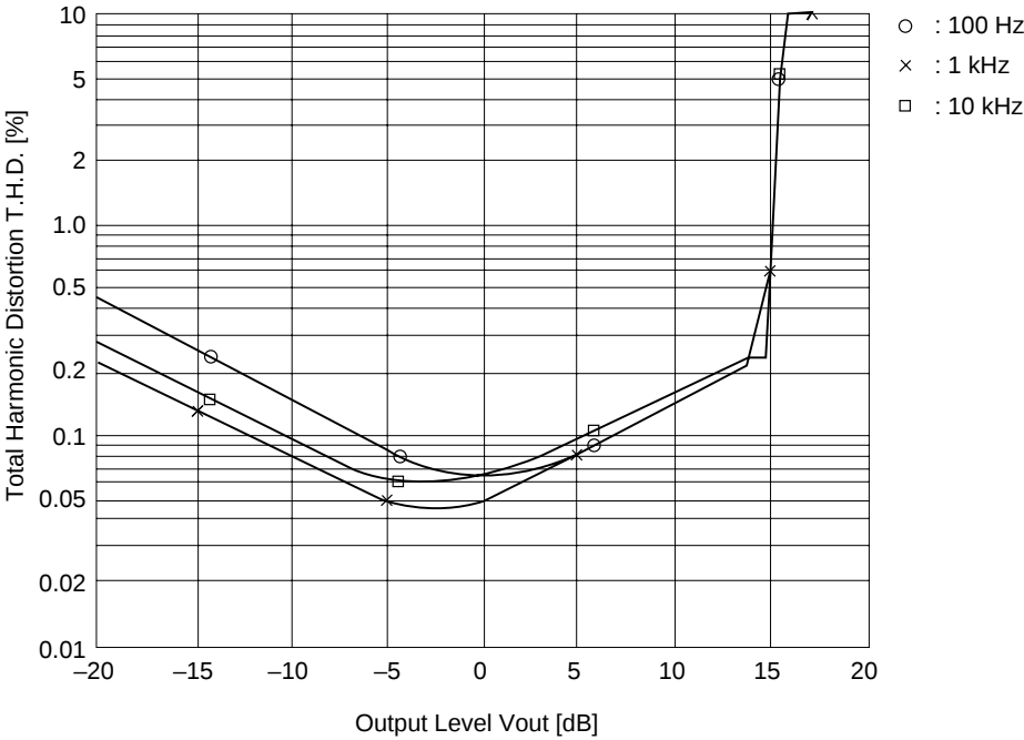
Total Harmonic Distortion vs. Output Level (PB MODE NR-OFF V CC = 14 V)
