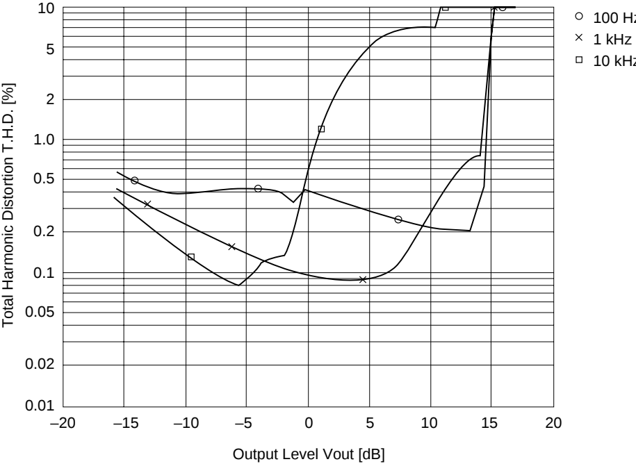
Total Harmonic Distortion vs. Output Level (REC MODE NR-C V CC = 14 V)
