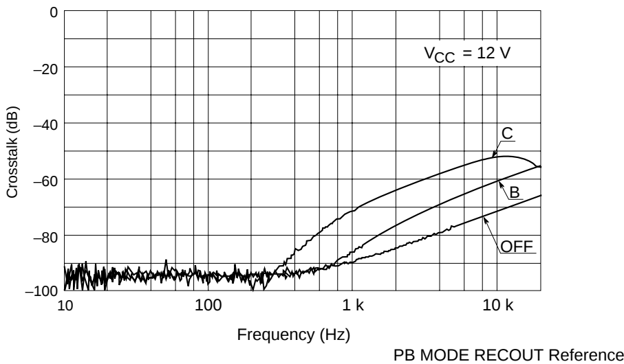
Crosstalk vs. Frequency (PB→REC)
