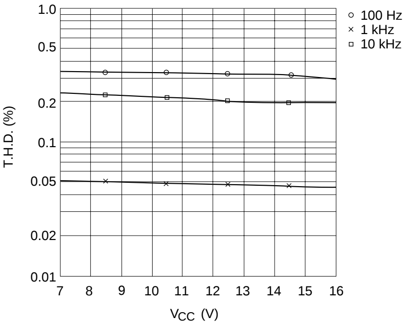
Total Harmonic Distortion vs. Supply Voltage (PB MODE NR-C)
