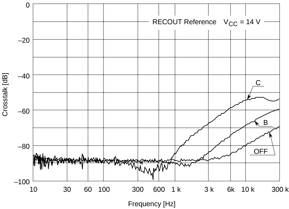
Crosstalk vs. Frequency (REC MODE R↔L)
