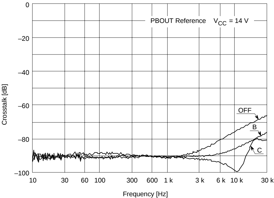
Crosstalk vs. Frequency (PB MODE R↔L)
