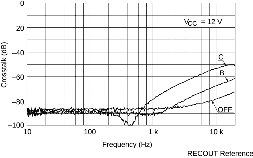
Crosstalk vs. Frequency (REC MODE R→L)
