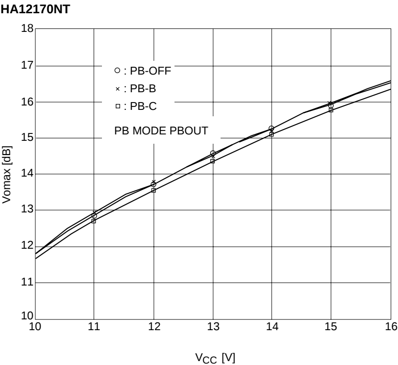
Maximum Output Level vs. Supply Voltage
