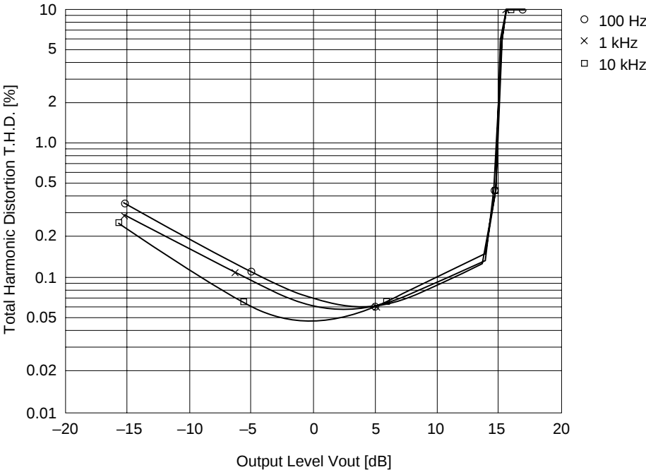
Total Harmonic Distortion vs. Output Level (REC MODE NR-B V CC = 14 V)
