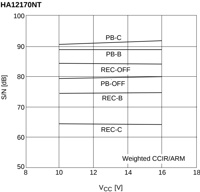
S/N vs. Supply Voltage
