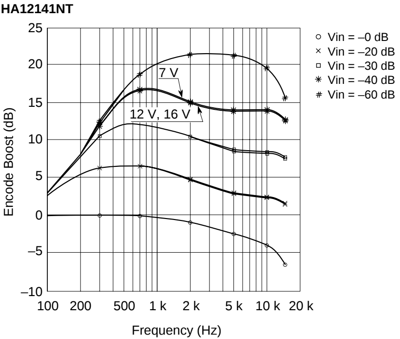
Encode Boost vs. Frequency (NR-C V_{CC} = 7\text{ V}, 12\text{ V}, 16\text{ V} )
