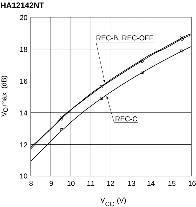
Maximum Output Level vs. Supply Voltage (REC MODE)
