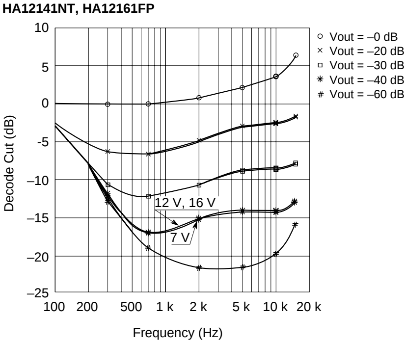
Decode Cut vs Frequency (NR-C V_{CC} = 7 V, 12 V, 16 V)
