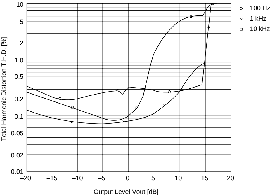
Total Harmonic Distortion vs. Output Level (PB MODE NR-C V CC = 14 V)
