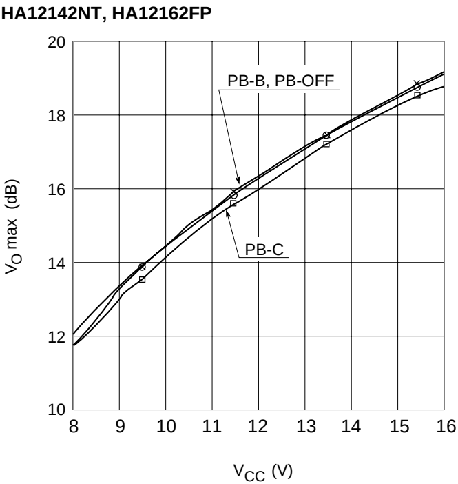
Maximum Output Level vs. Supply Voltage (PB MODE)
