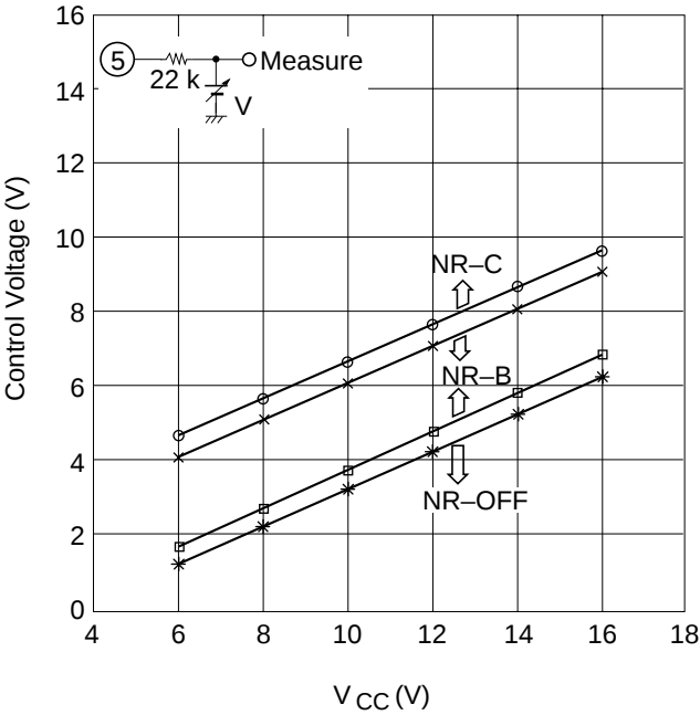
Control Voltage vs. Supply voltage (NR-OFF/B/C)
