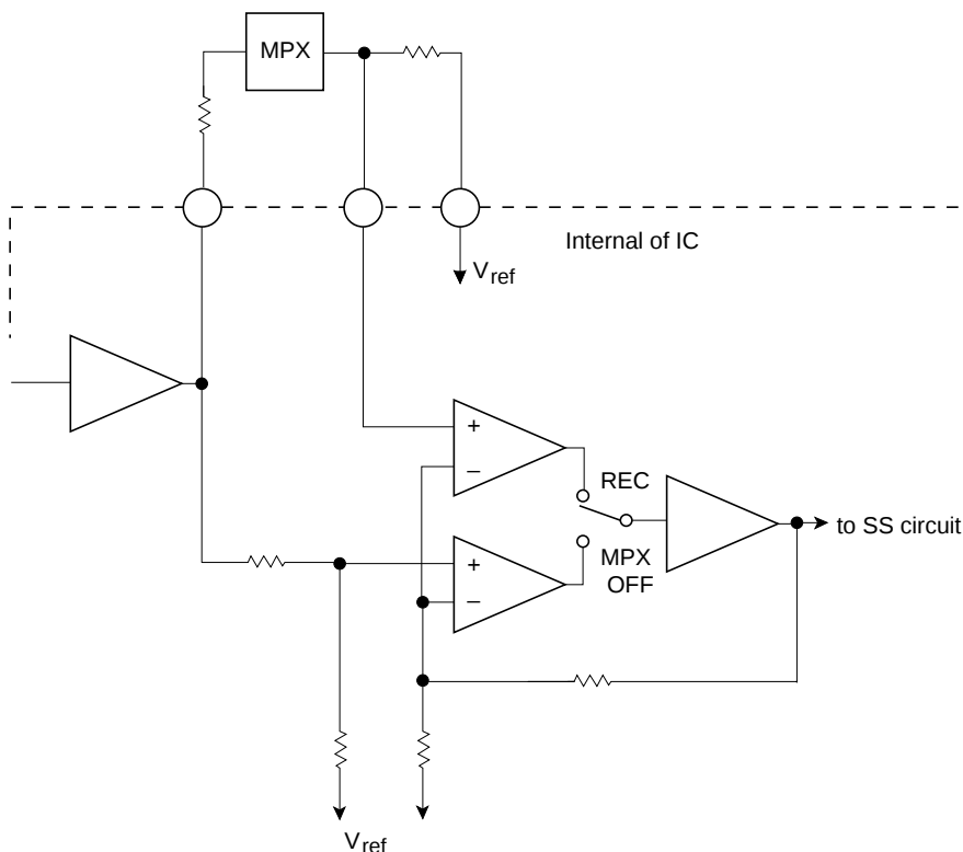
Figure 2 The Block-Diagram of MPX Driving Circuit
