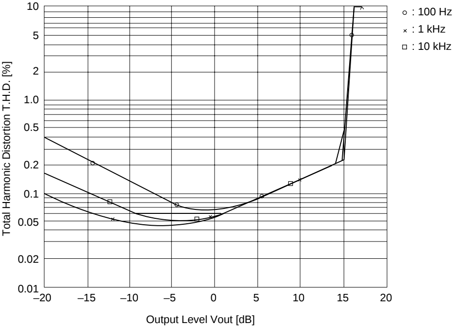
Total Harmonic Distortion vs. Output Level (PB MODE NR-B V CC = 14 V)
