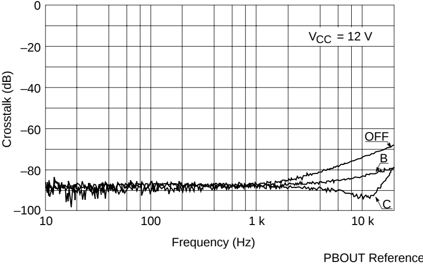
Crosstalk vs. Frequency (PB MODE R→L)
