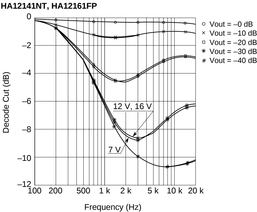
Decode Cut vs. Frequency (NR-B V_{CC} = 7\text{ V}, 12\text{ V}, 16\text{ V} )
