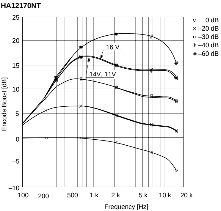
Encode Boost vs. Frequency (NR-C V_{CC} = 11\text{ V}, 14\text{ V}, 16\text{ V} )
