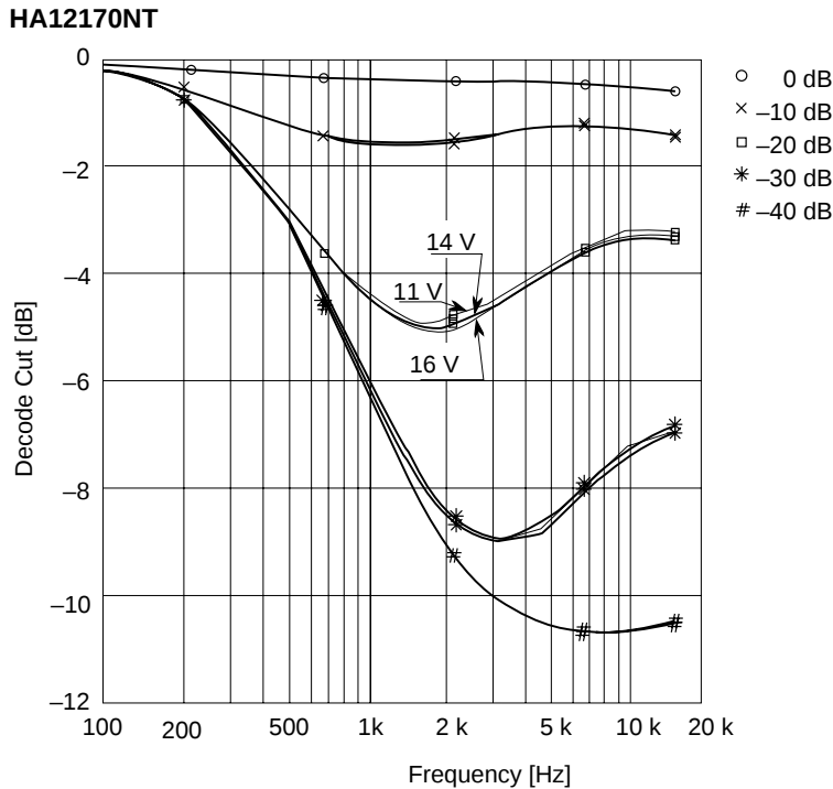
Decode Cut vs. Frequency (NR-B V_{CC} = 11\text{ V}, 14\text{ V}, 16\text{ V} )
