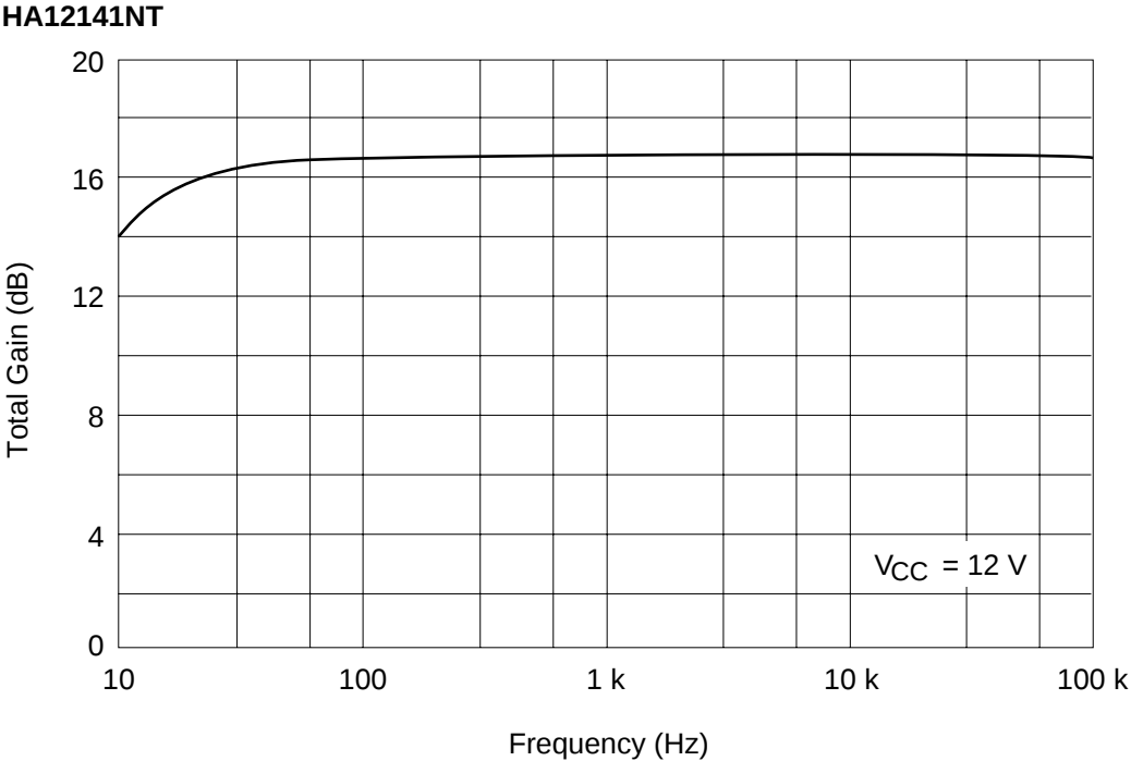
Total Gain vs. Frequency (REC MODE RECOUT NR-OFF)
