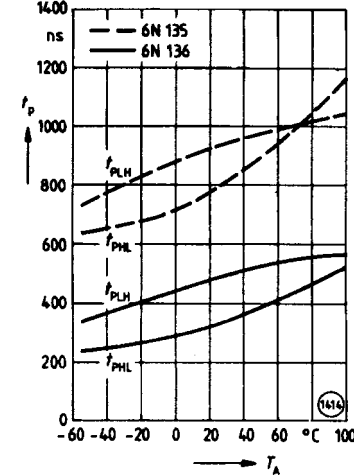
Figure 12. Delay Times vs. Ambient Temperature I_F=16\text{ mA} , V_{CC}=5.0\text{ V} , R_L=4.1\text{ k}\Omega , SFH636: R_L=1.9\text{ k}\Omega
