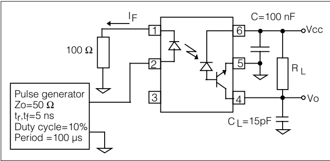
Figure 1. Test Set-up
