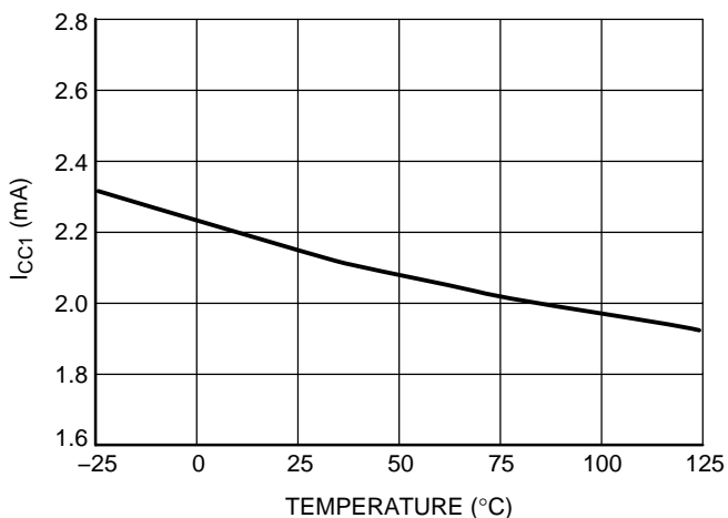
Figure 12. No Load Circuit Consumption vs. Temperature
