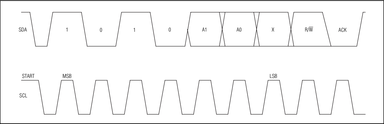
Figure 7. Slave Address
