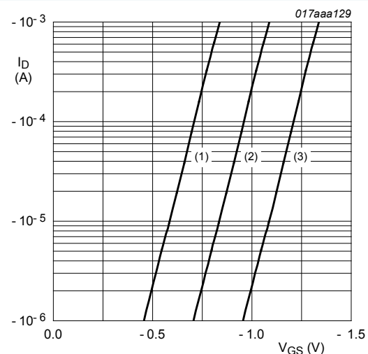
Fig. 7. Sub-threshold drain current as a function of gate-source voltage T_j = 25\text{ }^{\circ}\text{C}; V_{DS} = -3\text{ V} (1) minimum values (2) typical values (3) maximum values
