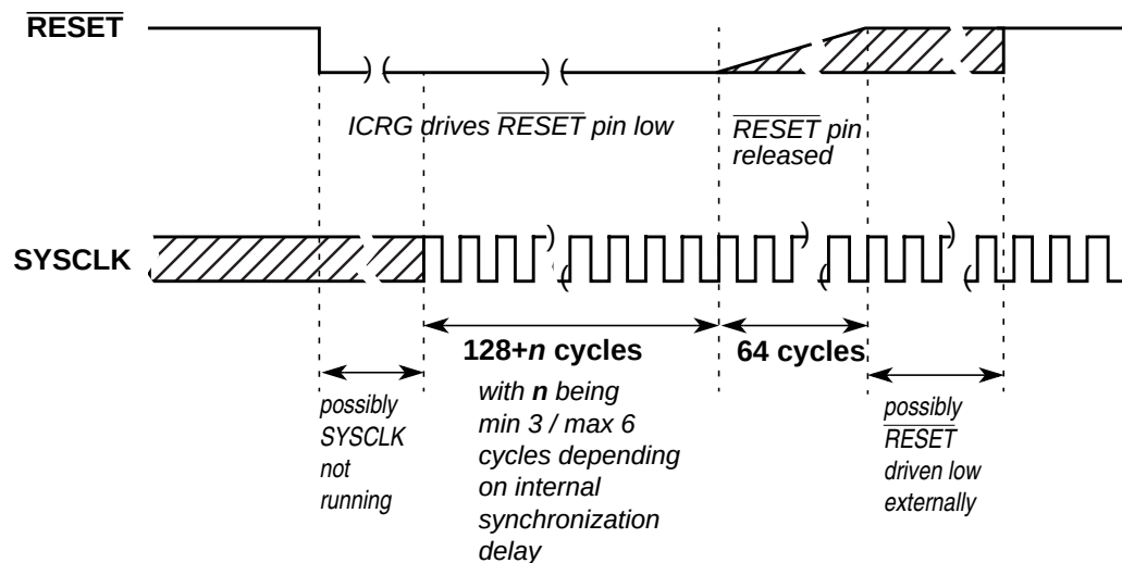
Figure 8-21. RESET Timing
