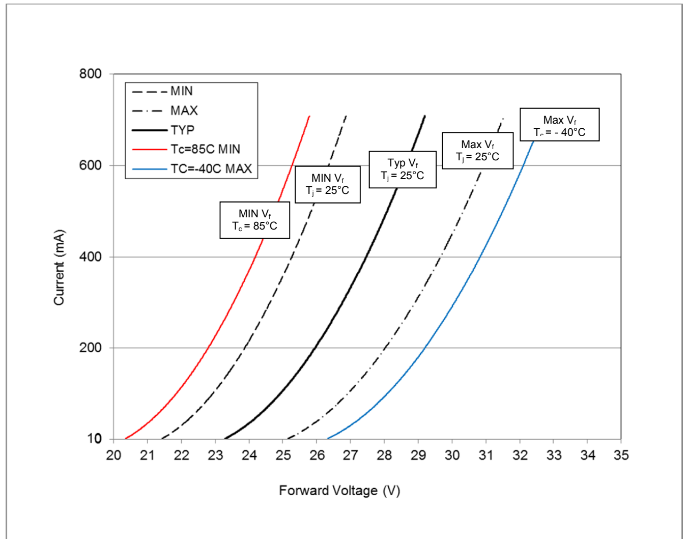
Figure 1: Electrical Characteristics
