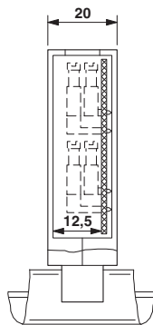
Dimensioned drawing
