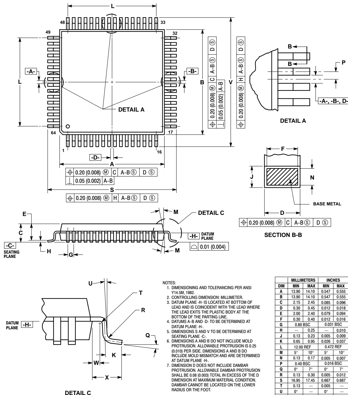
Figure 23-1. MC68HC908MR32FU
