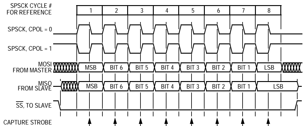
Figure 13-6. Transmission Format ( \text{CPHA} = 1 )
