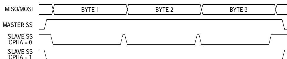
Figure 13-5. CPHA/ \overline{\text{SS}} Timing
