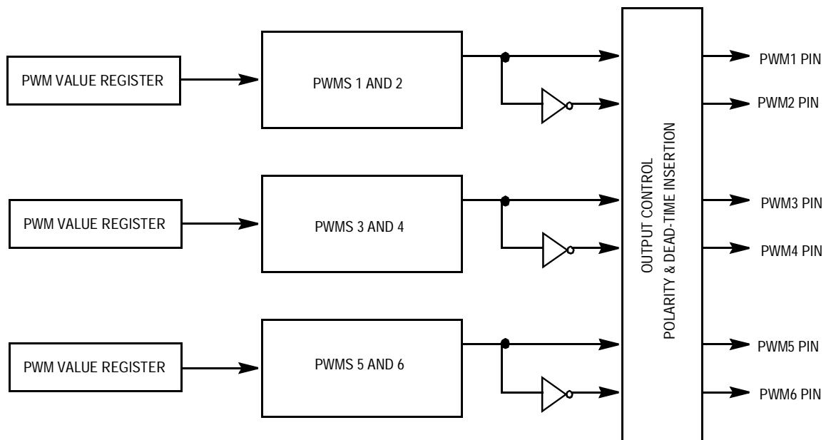
Figure 9-11. Complementary Pairing
