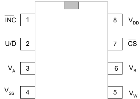
8-SOIC
