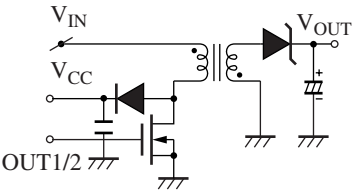
Figure 1. Output bootstrap circuit
