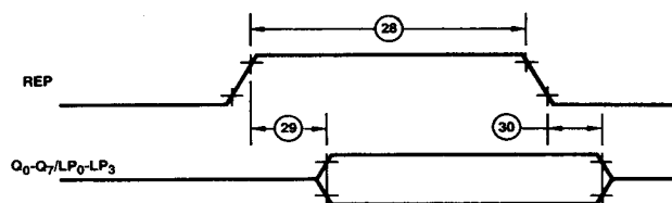
Figure 15. Read Error Pattern Timing
