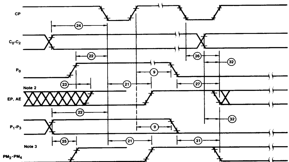
Figure 14. Timing for Correct High-Speed Function
